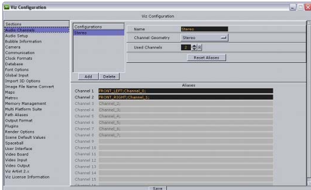
Figure 104: Viz Configuration interface, Video
