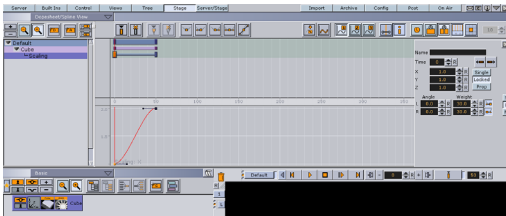
Figure 77: Example of animation where Cube container is scaled at field 0 and 50
