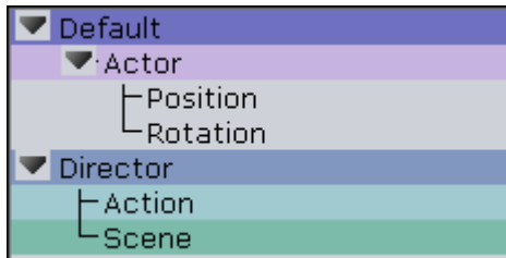
Figure 56: Stage tree with directors, actor, channels, action, and scene
