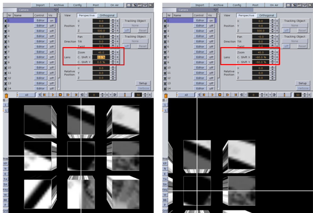
Figure 102: Left is default (0); right is C Shift X = -60 and C Shift Y = -60
