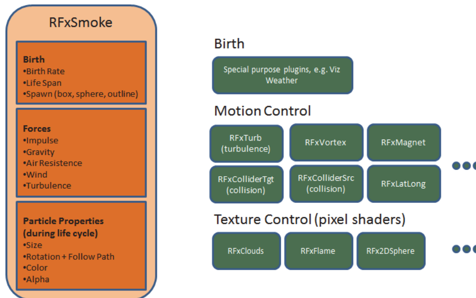
Figure 12: RealFX Architecture
