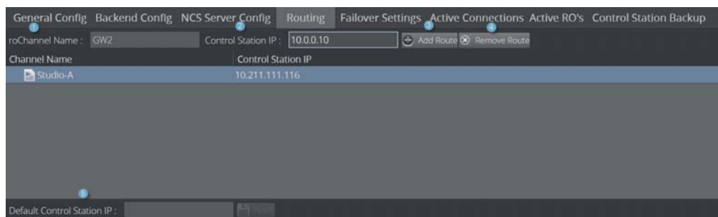
Figure 2: Routing
